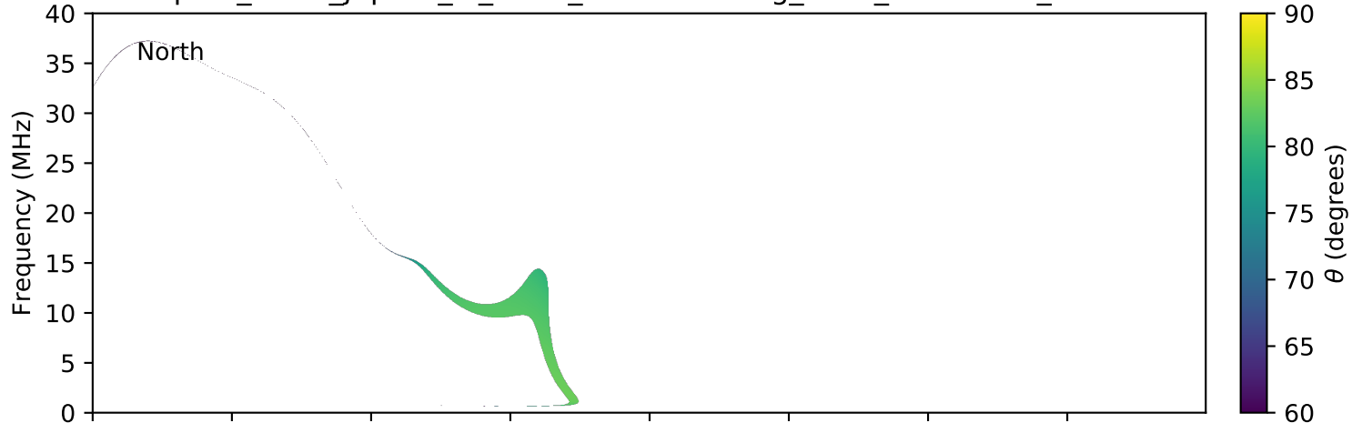
expres_earth_jupiter_io_isaac_lossc-wid1deg_3kev_20160308_v01.cdf
