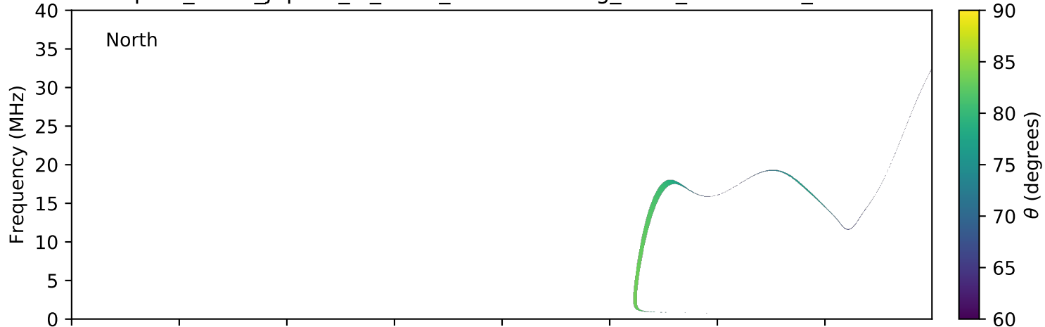
expres_earth_jupiter_io_isaac_lossc-wid1deg_3kev_20160307_v01.cdf
