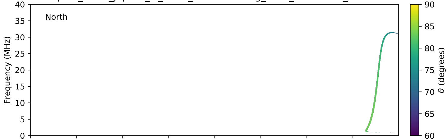
expres_earth_jupiter_io_isaac_lossc-wid1deg_3kev_20160305_v01.cdf
