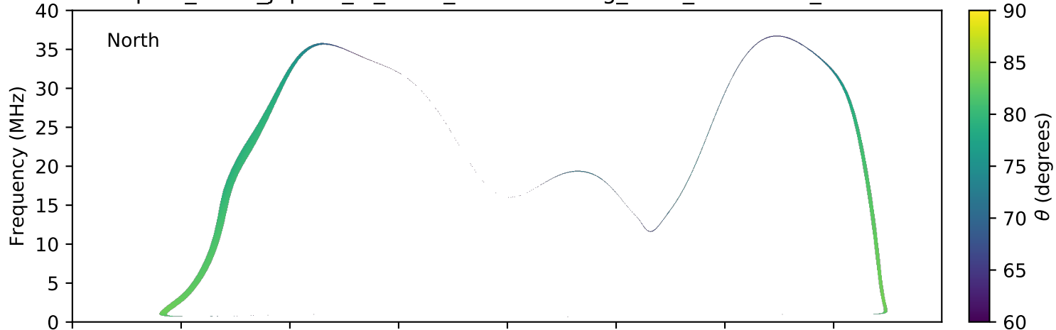
expres_earth_jupiter_io_isaac_lossc-wid1deg_3kev_20160304_v01.cdf
