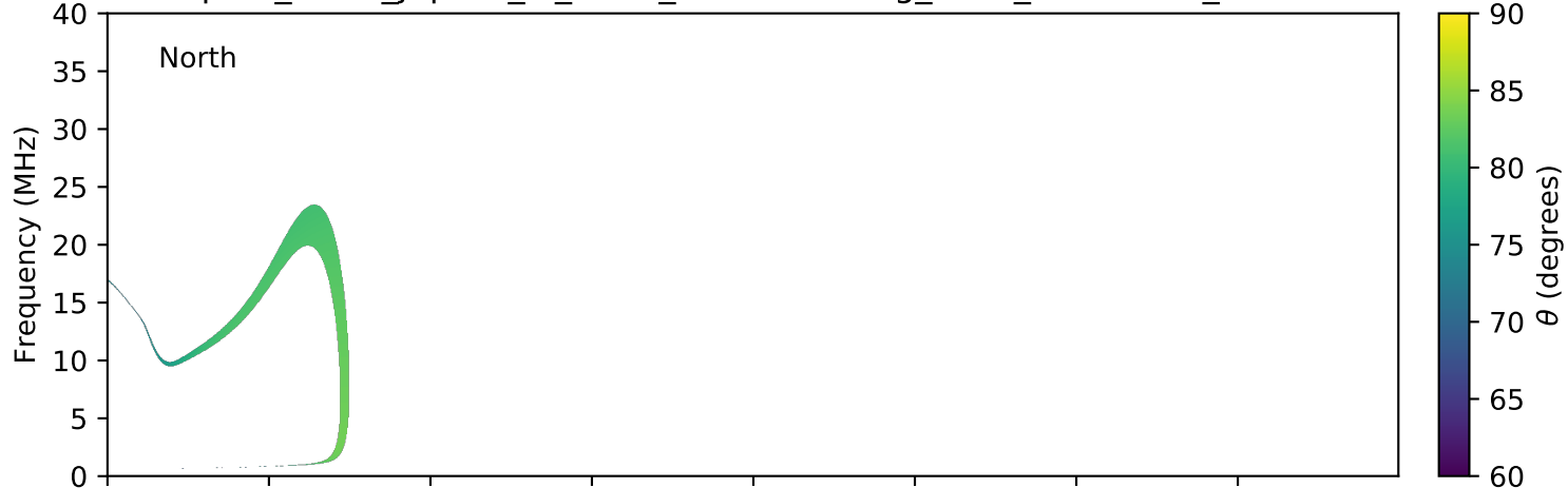
expres_earth_jupiter_io_isaac_lossc-wid1deg_3kev_20160303_v01.cdf
