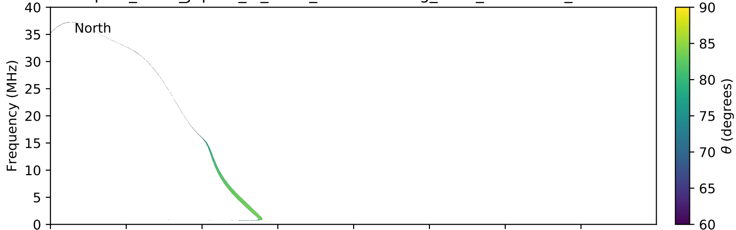
expres_earth_jupiter_io_isaac_lossc-wid1deg_3kev_20160301_v01.cdf
