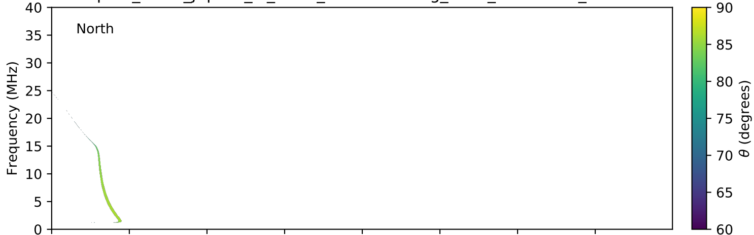
expres_earth_jupiter_io_isaac_lossc-wid1deg_1kev_20160326_v01.cdf
