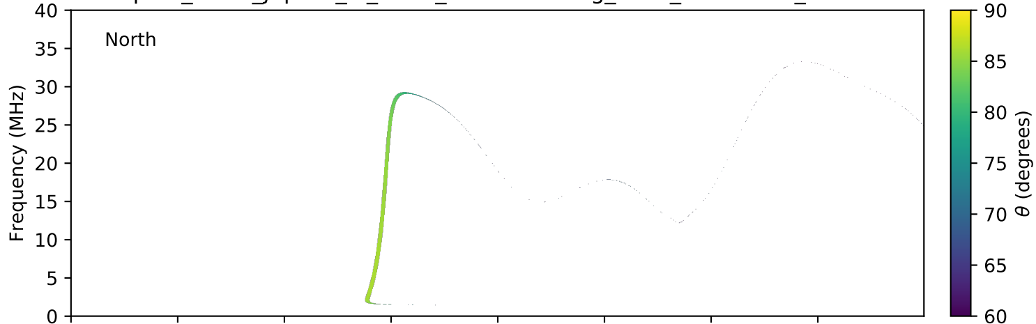
expres_earth_jupiter_io_isaac_lossc-wid1deg_1kev_20160325_v01.cdf
