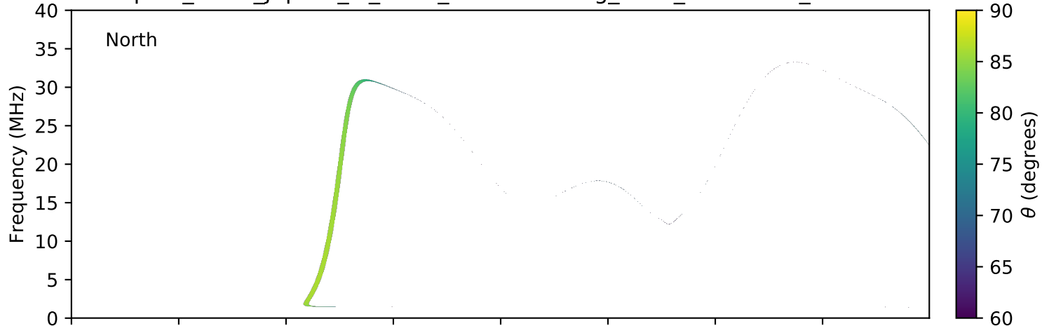
expres_earth_jupiter_io_isaac_lossc-wid1deg_1kev_20160318_v01.cdf
