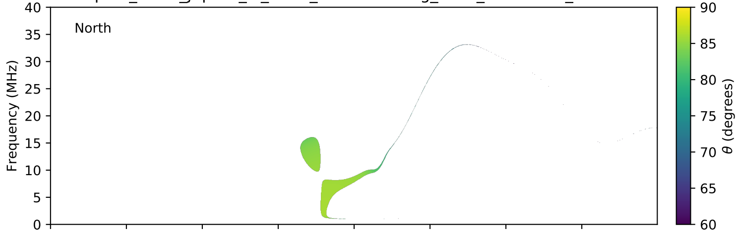
expres_earth_jupiter_io_isaac_lossc-wid1deg_1kev_20160316_v01.cdf
