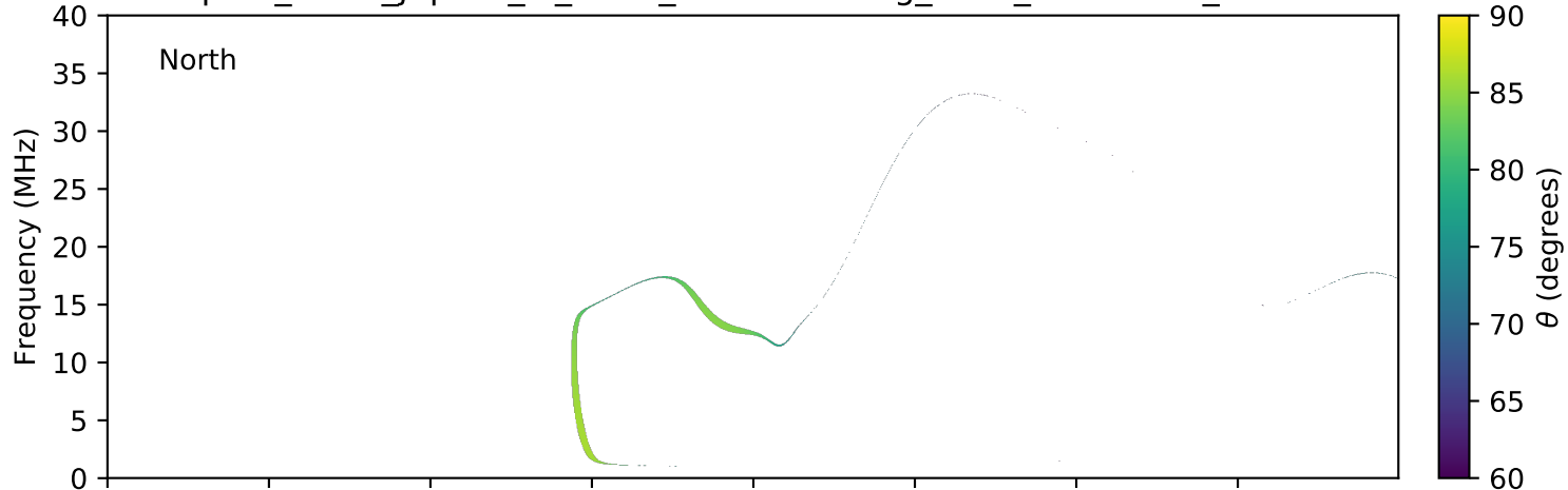
expres_earth_jupiter_io_isaac_lossc-wid1deg_1kev_20160309_v01.cdf
