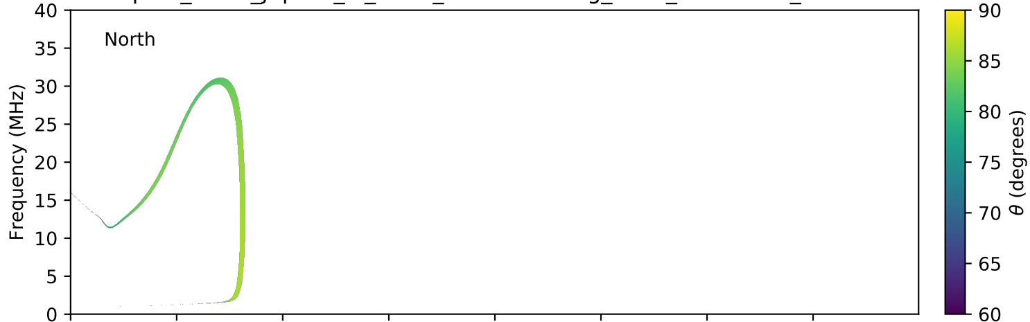
expres_earth_jupiter_io_isaac_lossc-wid1deg_1kev_20160303_v01.cdf
