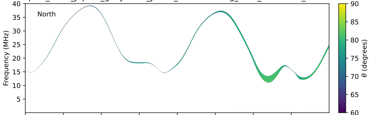
expres_earth_jupiter_ganymede_jrm33_lossc-wid1deg_3kev_20160310_v11.cdf
