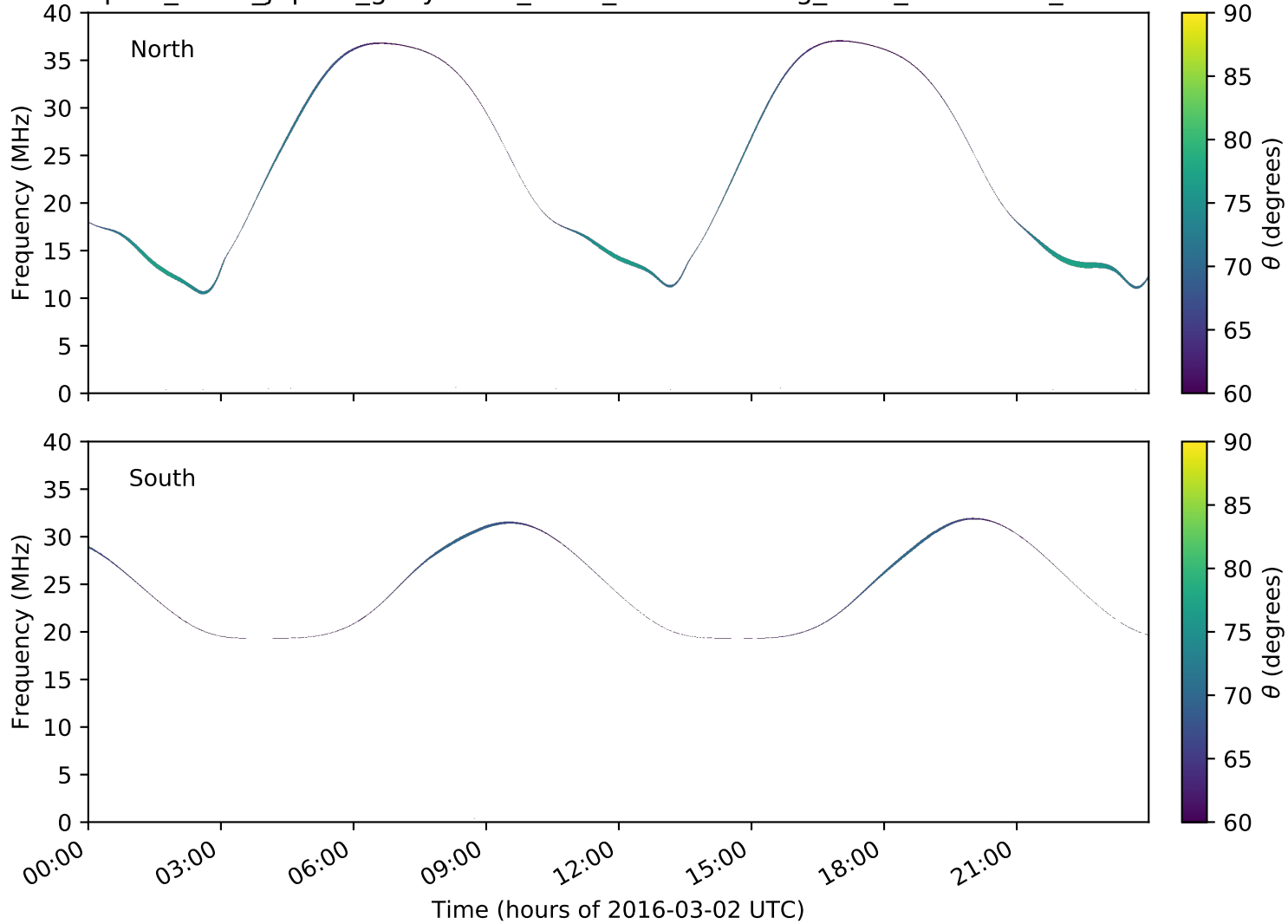
expres_earth_jupiter_ganymede_isaac_lossc-wid1deg_5kev_20160302_v01.cdf
