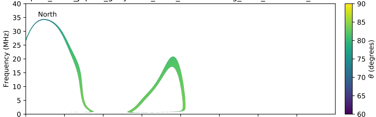
expres_earth_jupiter_ganymede_isaac_lossc-wid1deg_3kev_20160318_v01.cdf
