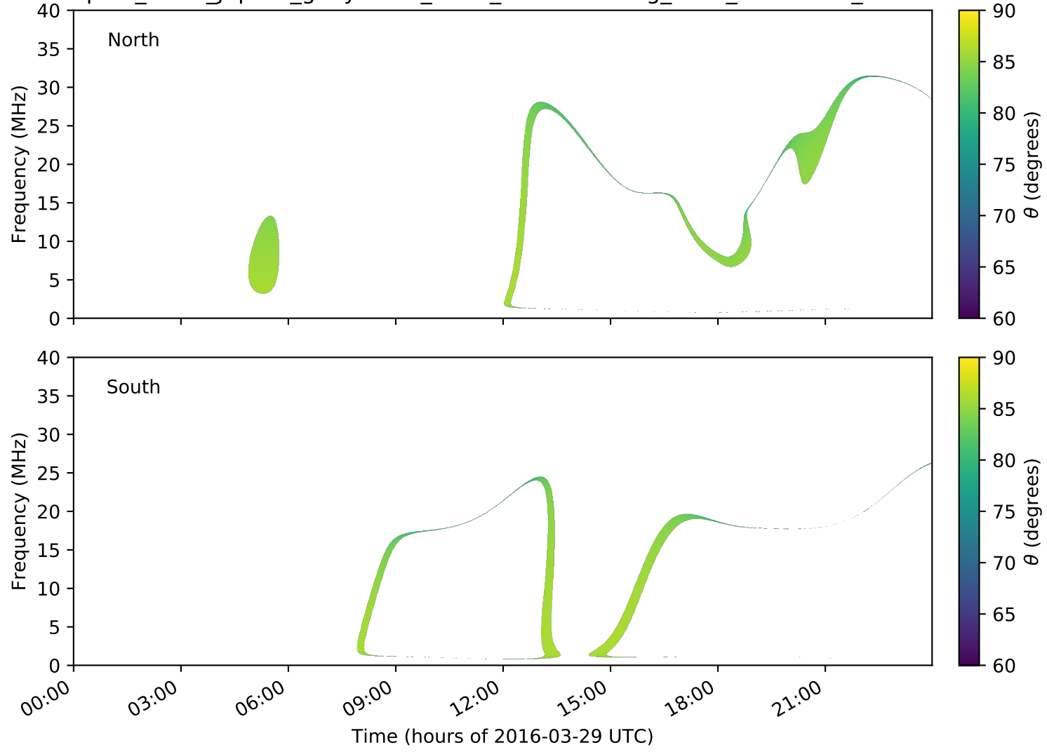
expres_earth_jupiter_ganymede_isaac_lossc-wid1deg_1kev_20160329_v01.cdf
