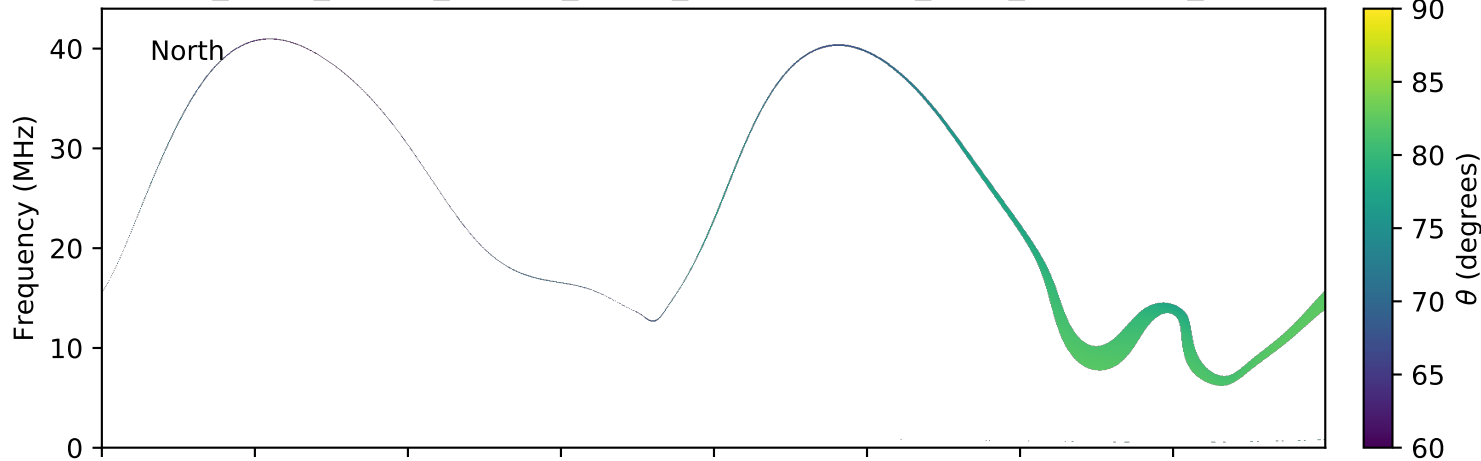
expres_earth_jupiter_europa_jrm09_lossc-wid1deg_3kev_20160322_v01.cdf
