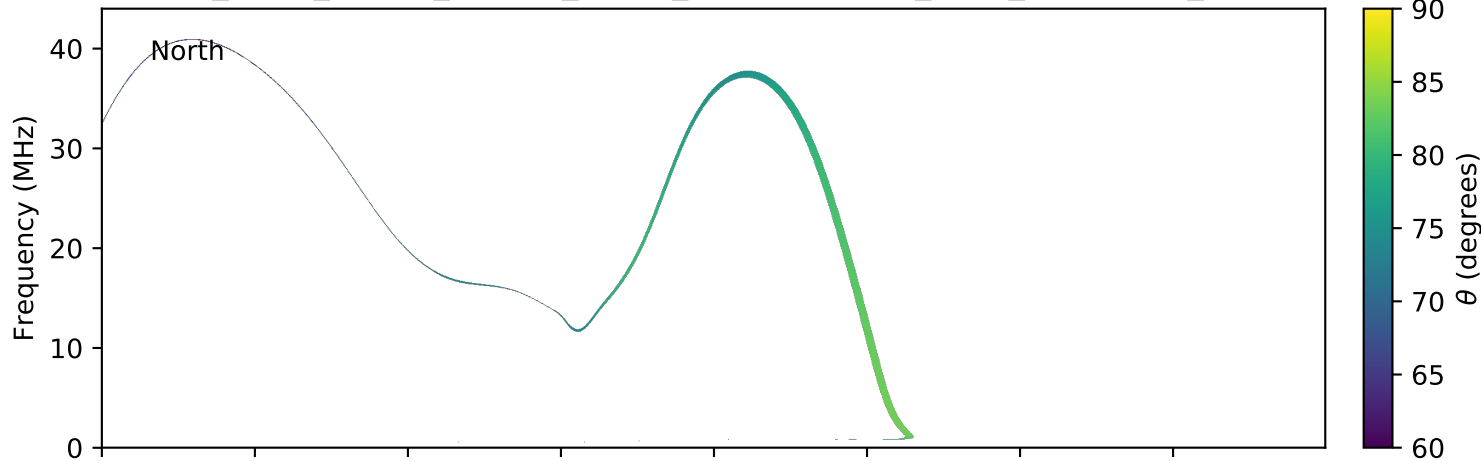
expres_earth_jupiter_europa_jrm09_lossc-wid1deg_3kev_20160301_v01.cdf
