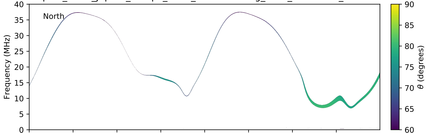
expres_earth_jupiter_europa_isaac_lossc-wid1deg_5kev_20160329_v01.cdf
