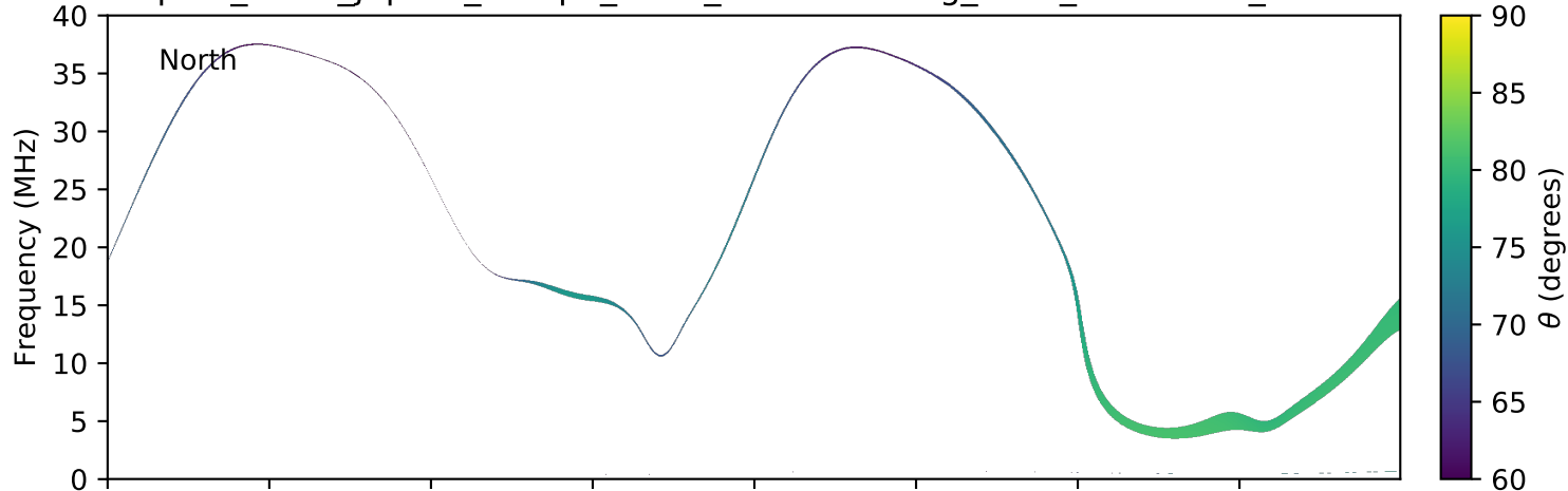
expres_earth_jupiter_europa_isaac_lossc-wid1deg_5kev_20160322_v01.cdf
