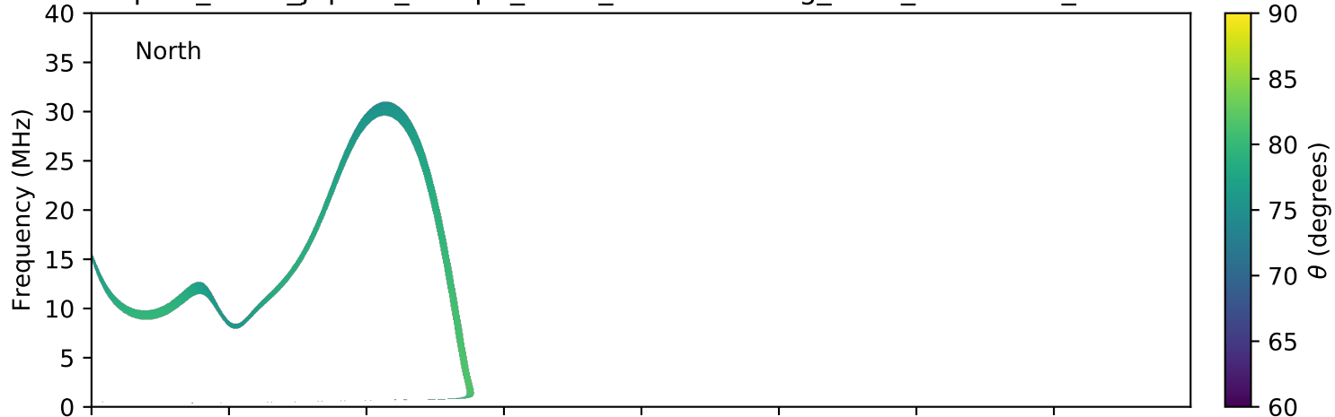
expres_earth_jupiter_europa_isaac_lossc-wid1deg_5kev_20160312_v01.cdf
