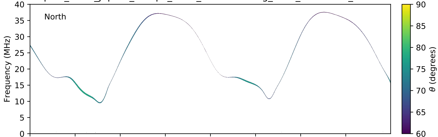
expres_earth_jupiter_europa_isaac_lossc-wid1deg_5kev_20160311_v01.cdf
