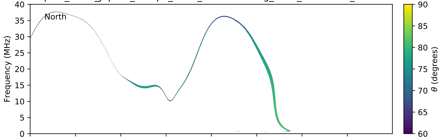
expres_earth_jupiter_europa_isaac_lossc-wid1deg_5kev_20160308_v01.cdf
