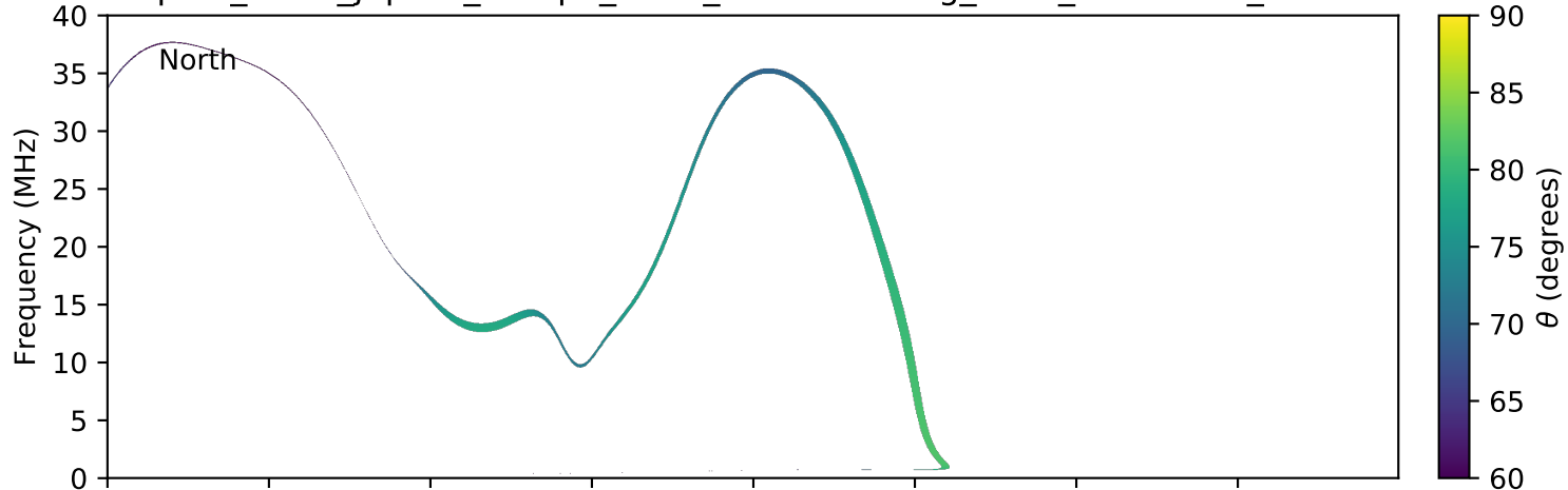
expres_earth_jupiter_europa_isaac_lossc-wid1deg_5kev_20160301_v01.cdf
