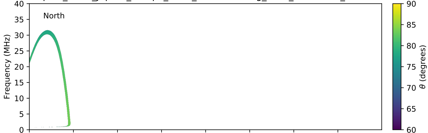
expres_earth_jupiter_europa_isaac_lossc-wid1deg_3kev_20160330_v01.cdf
