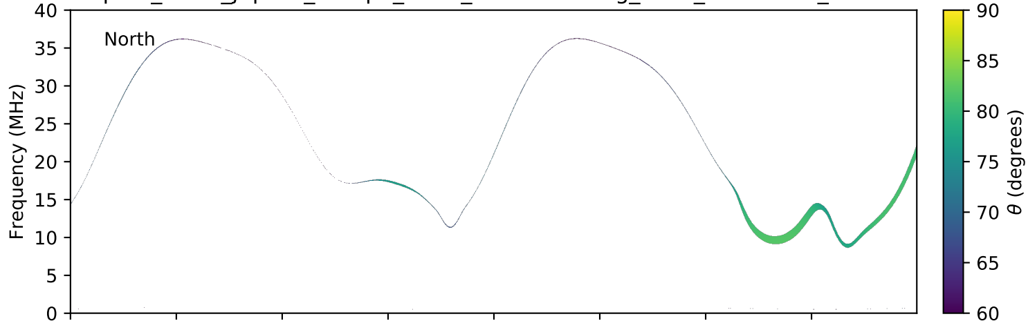
expres_earth_jupiter_europa_isaac_lossc-wid1deg_3kev_20160329_v01.cdf
