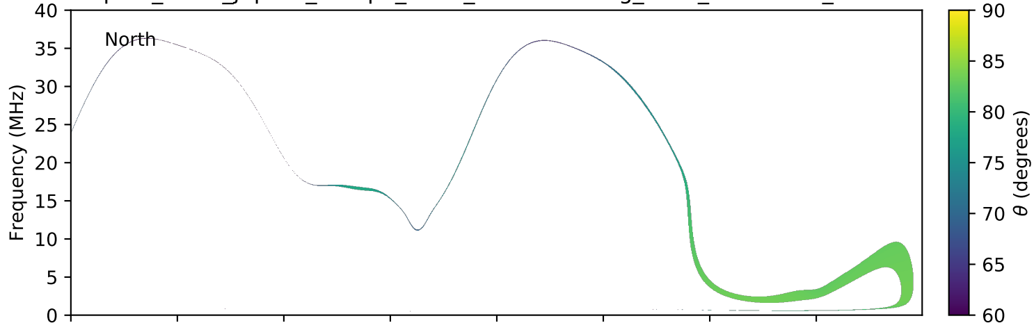
expres_earth_jupiter_europa_isaac_lossc-wid1deg_3kev_20160315_v01.cdf
