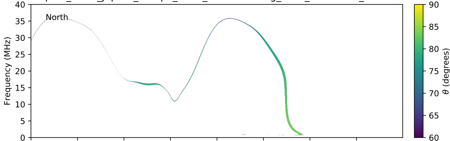
expres_earth_jupiter_europa_isaac_lossc-wid1deg_3kev_20160308_v01.cdf
