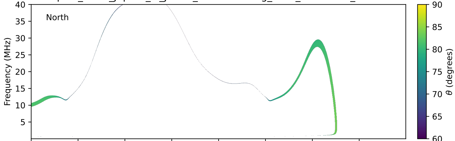
expres_earth_jupiter_io_jrm33_lossc-wid1deg_3kev_20160219_v11.cdf
