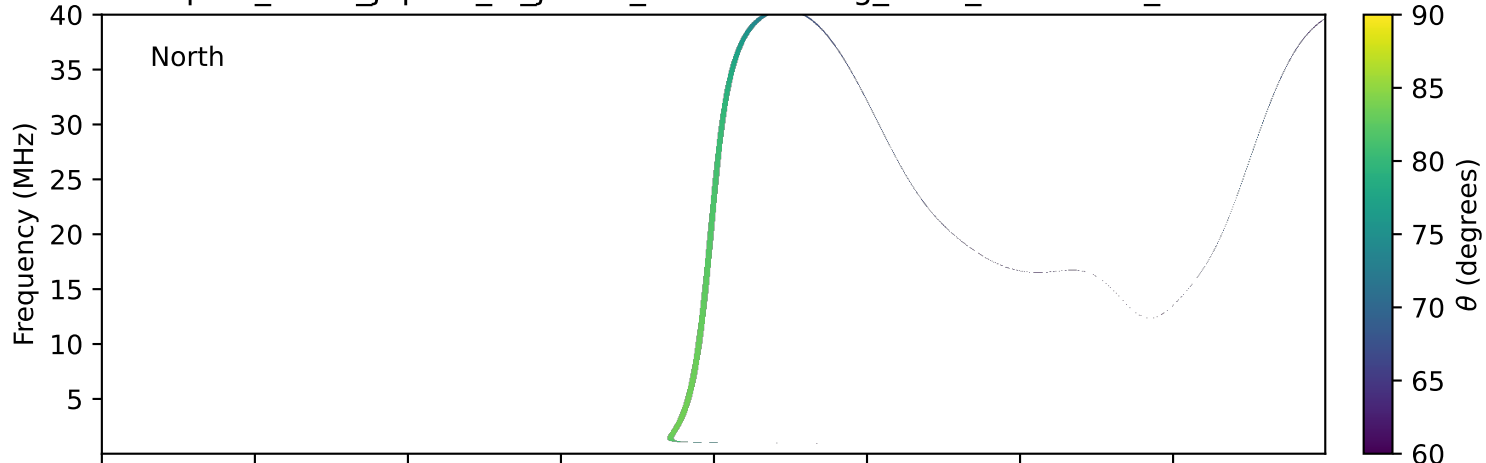
expres_earth_jupiter_io_jrm33_lossc-wid1deg_3kev_20160215_v11.cdf
