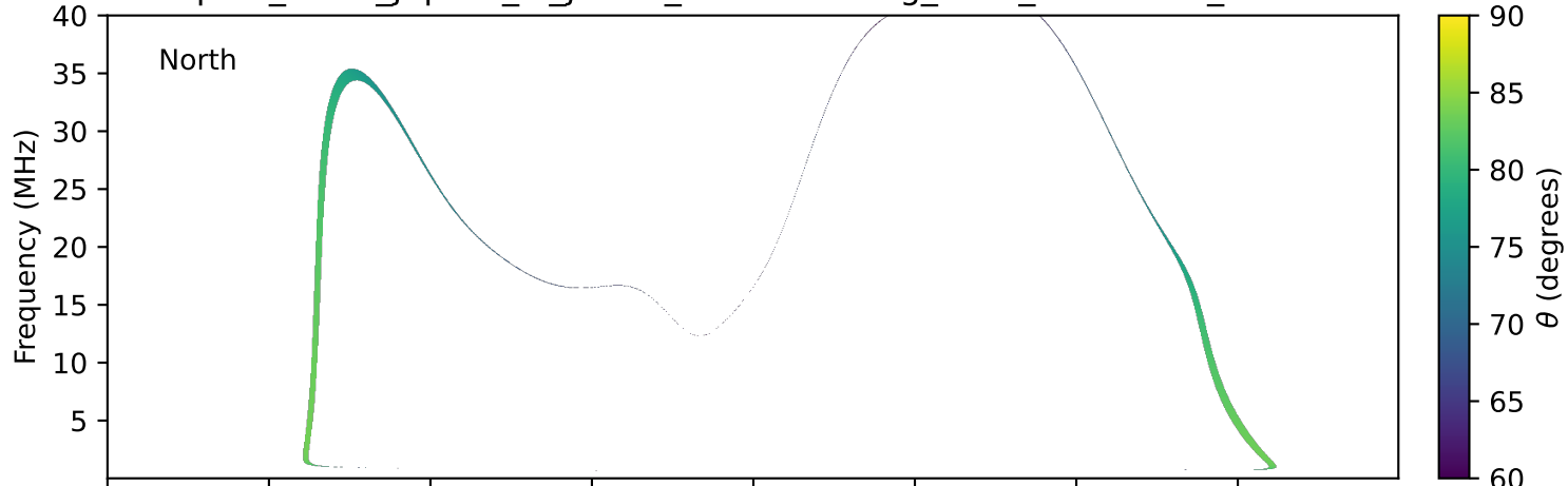
expres_earth_jupiter_io_jrm33_lossc-wid1deg_3kev_20160210_v11.cdf
