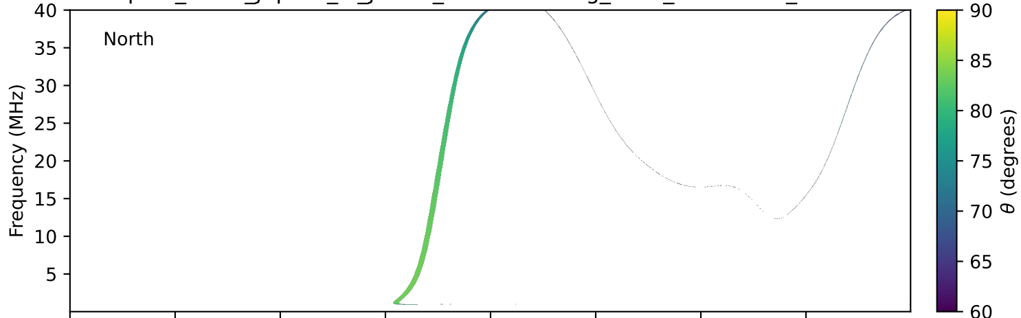
expres_earth_jupiter_io_jrm33_lossc-wid1deg_3kev_20160208_v11.cdf
