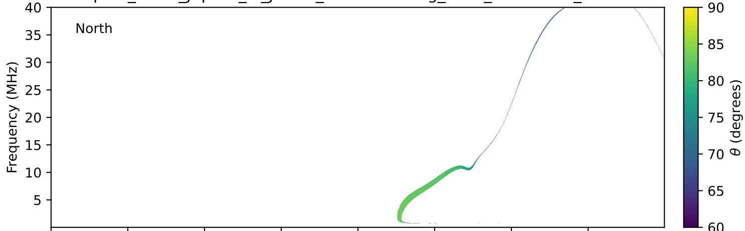
expres_earth_jupiter_io_jrm33_lossc-wid1deg_3kev_20160206_v11.cdf
