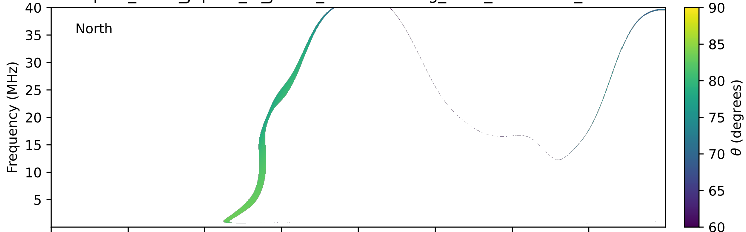
expres_earth_jupiter_io_jrm33_lossc-wid1deg_3kev_20160201_v11.cdf
