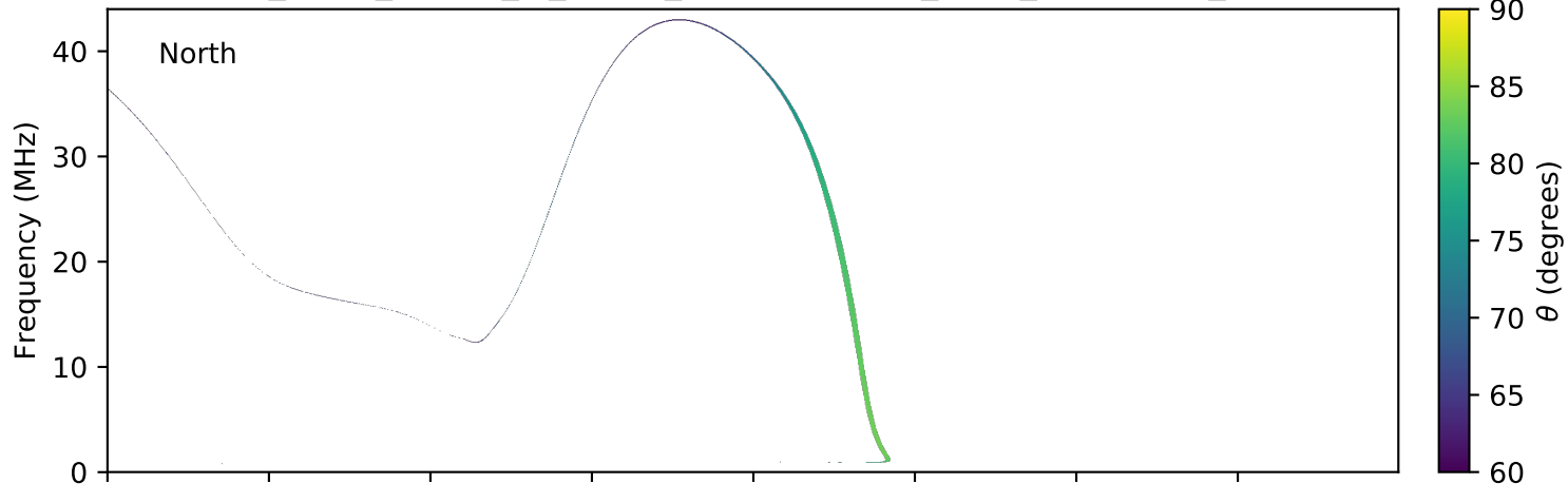
expres_earth_jupiter_io_jrm09_lossc-wid1deg_3kev_20160228_v01.cdf
