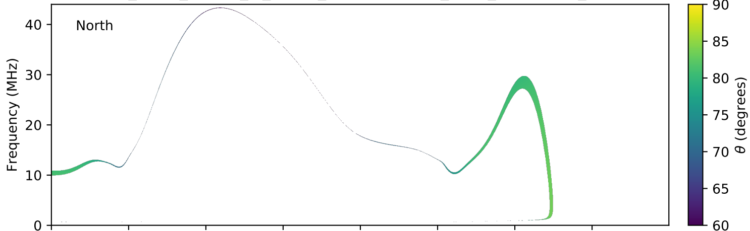
expres_earth_jupiter_io_jrm09_lossc-wid1deg_3kev_20160219_v01.cdf
