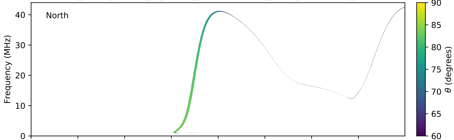
expres_earth_jupiter_io_jrm09_lossc-wid1deg_3kev_20160208_v01.cdf
