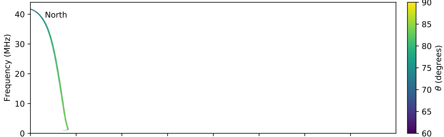
expres_earth_jupiter_io_jrm09_lossc-wid1deg_3kev_20160202_v01.cdf
