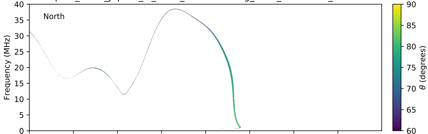
expres_earth_jupiter_io_isaac_lossc-wid1deg_5kev_20160228_v01.cdf
