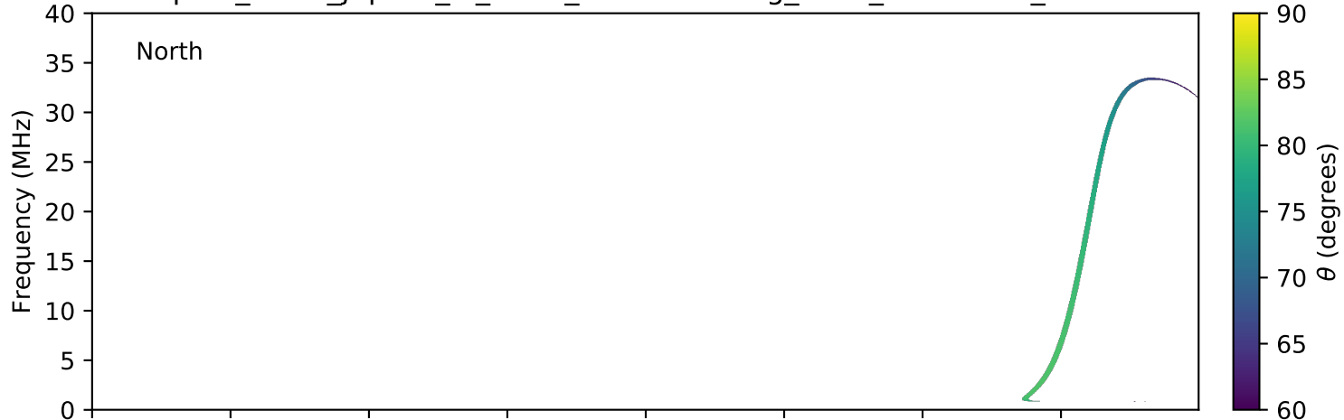
expres_earth_jupiter_io_isaac_lossc-wid1deg_5kev_20160227_v01.cdf
