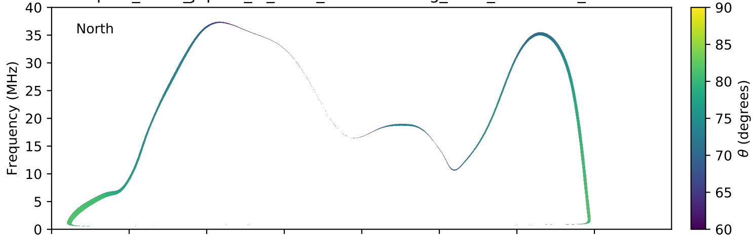
expres_earth_jupiter_io_isaac_lossc-wid1deg_5kev_20160226_v01.cdf
