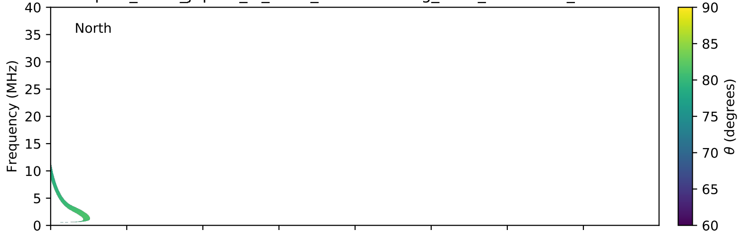
expres_earth_jupiter_io_isaac_lossc-wid1deg_5kev_20160225_v01.cdf
