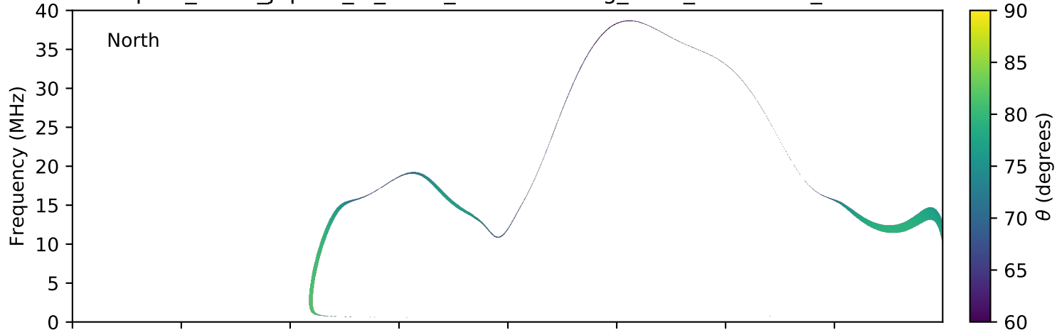
expres_earth_jupiter_io_isaac_lossc-wid1deg_5kev_20160224_v01.cdf
