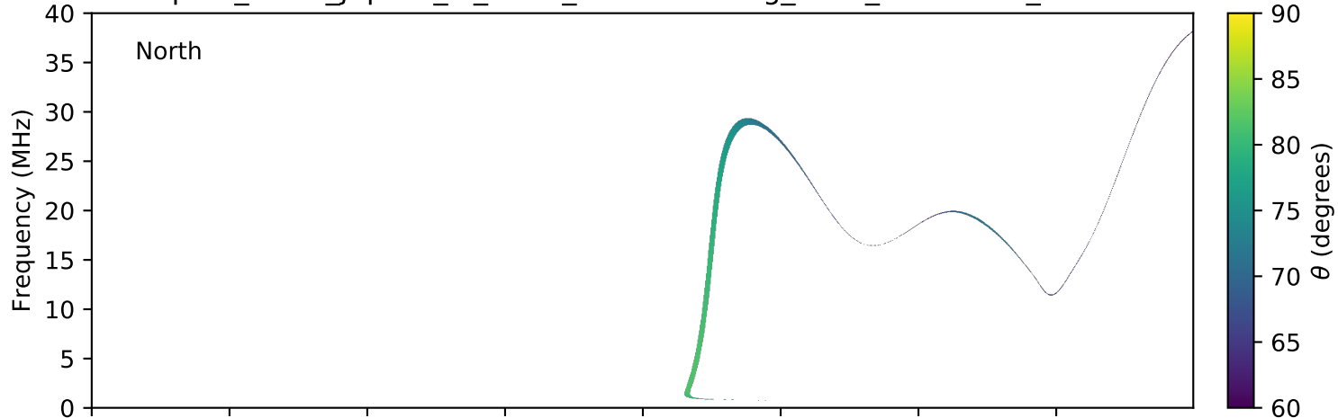
expres_earth_jupiter_io_isaac_lossc-wid1deg_5kev_20160222_v01.cdf
