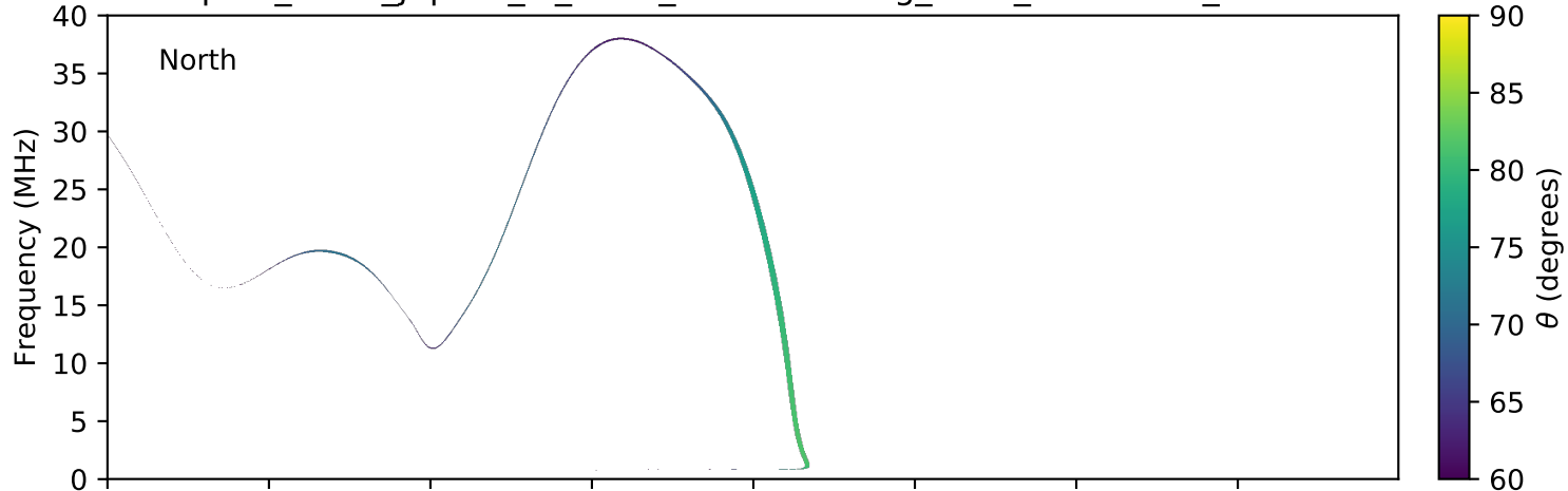
expres_earth_jupiter_io_isaac_lossc-wid1deg_5kev_20160221_v01.cdf
