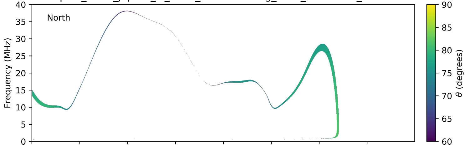
expres_earth_jupiter_io_isaac_lossc-wid1deg_5kev_20160219_v01.cdf
