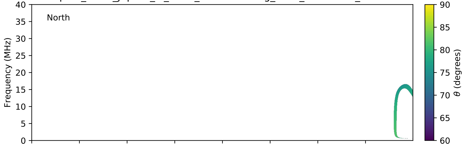
expres_earth_jupiter_io_isaac_lossc-wid1deg_5kev_20160218_v01.cdf
