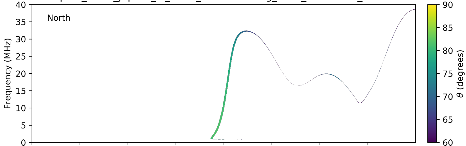
expres_earth_jupiter_io_isaac_lossc-wid1deg_5kev_20160215_v01.cdf
