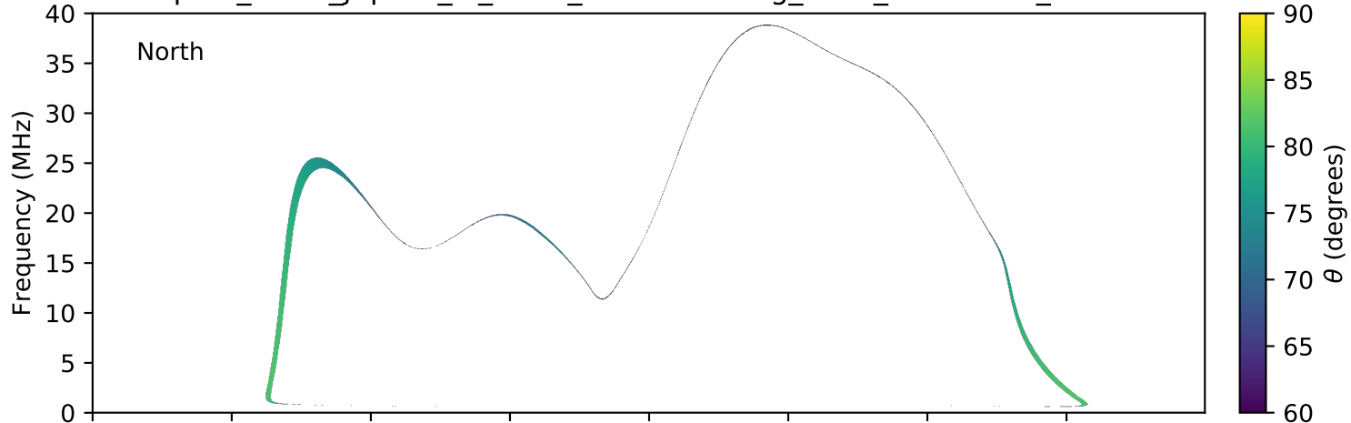
expres_earth_jupiter_io_isaac_lossc-wid1deg_5kev_20160210_v01.cdf
