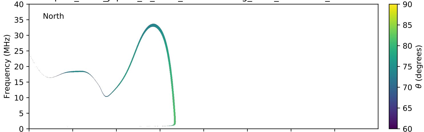
expres_earth_jupiter_io_isaac_lossc-wid1deg_5kev_20160207_v01.cdf
